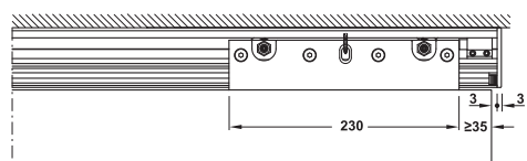
Section trolley hanger 80-120 kg
