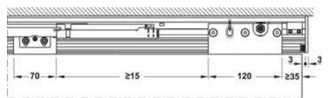
Section trolley hanger 40-50 kg with softclose mechanism
