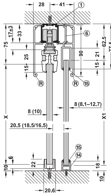
Ceiling installation with running track and clip panel 90 mm incl. fixed component. Sealing profile on one side for glass thickness 10 mm and wet sealing for glass thicknesses 8 – 12.7 mm
