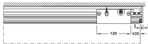
Section trolley hanger 40-50 kg
