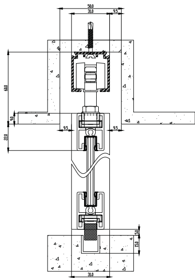
Hendren top track by ceiling design
