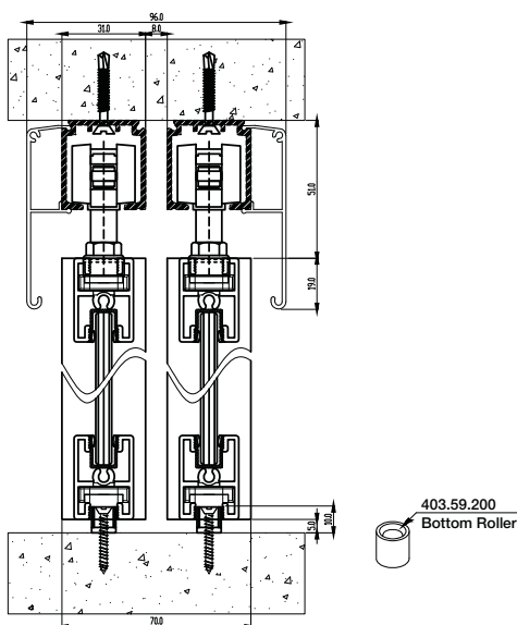
Bottom guide roller onto the floor
