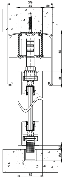
Twin side covers
