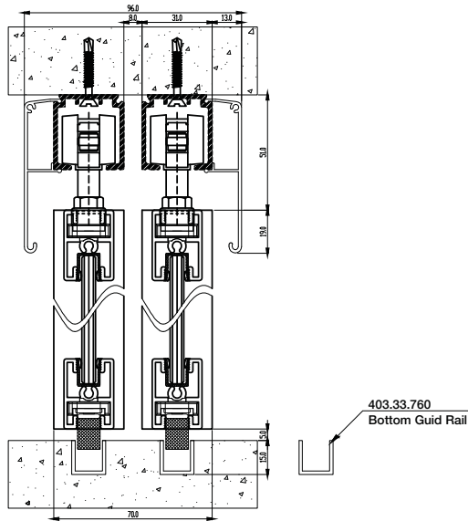
Standard bottom groove
