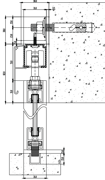
Single side cover onto the wall
