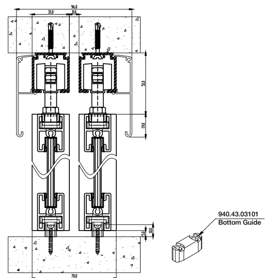
Bottom guide onto the floor
