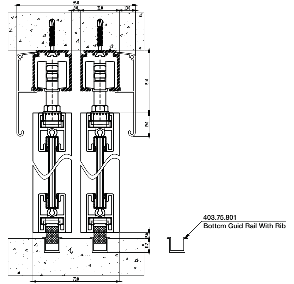
Special design bottom groove
