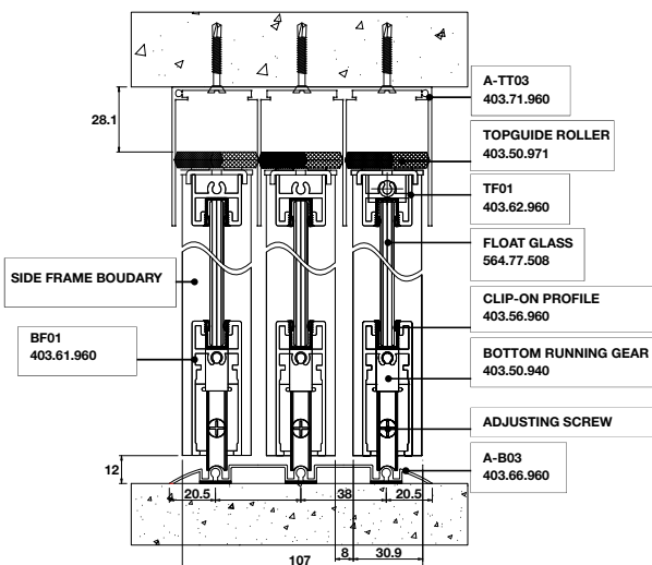
ALUFLEX BOTTOM RUNNING TRIPLE BOTTOM TRACK
