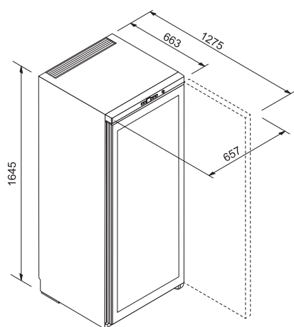
Installation Diagram
