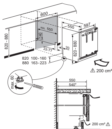
Installation Diagram
