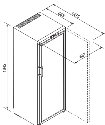
Installation Diagram
