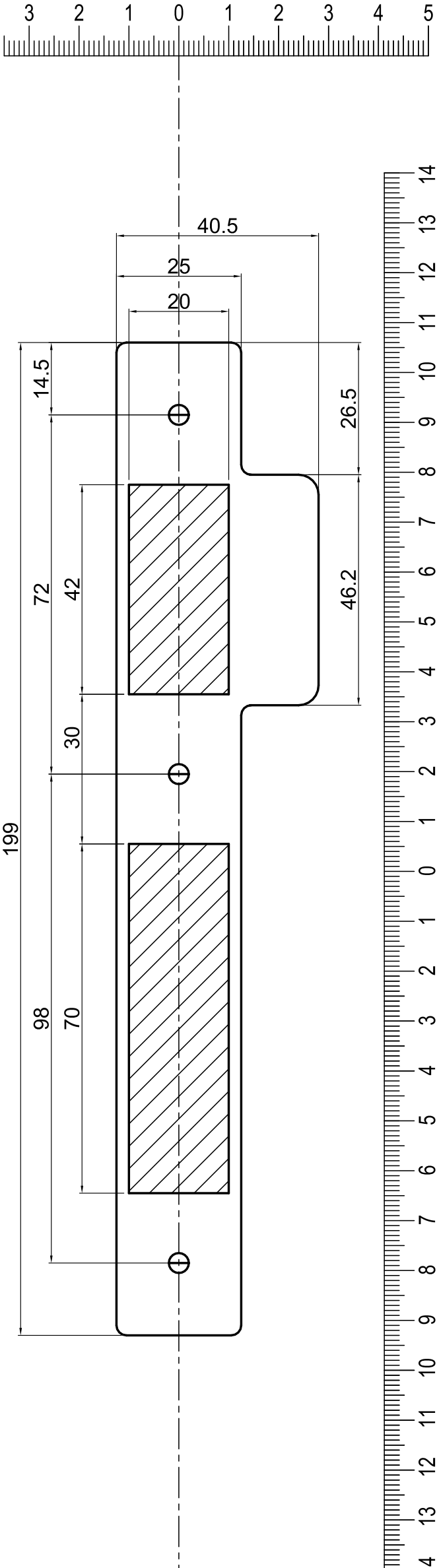
Template For Strike Plate
