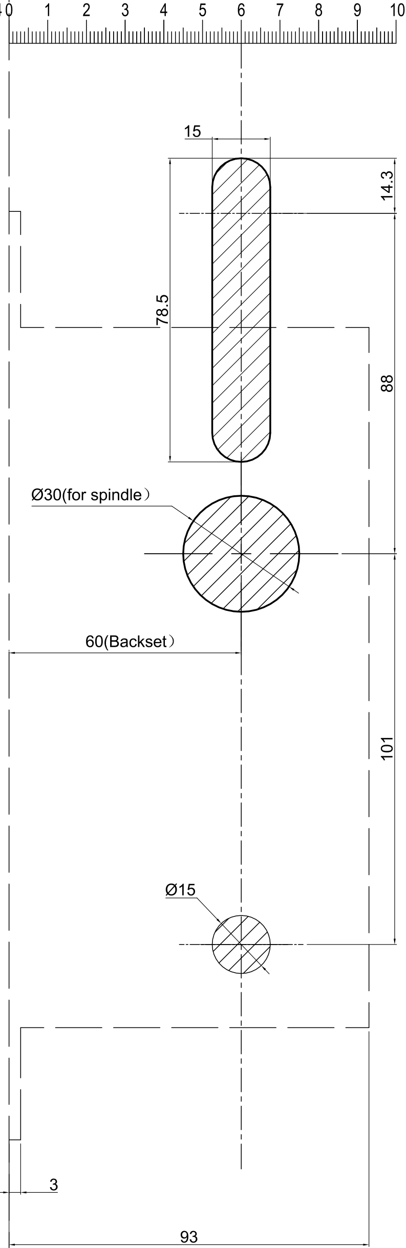
Template For Lock Panels
