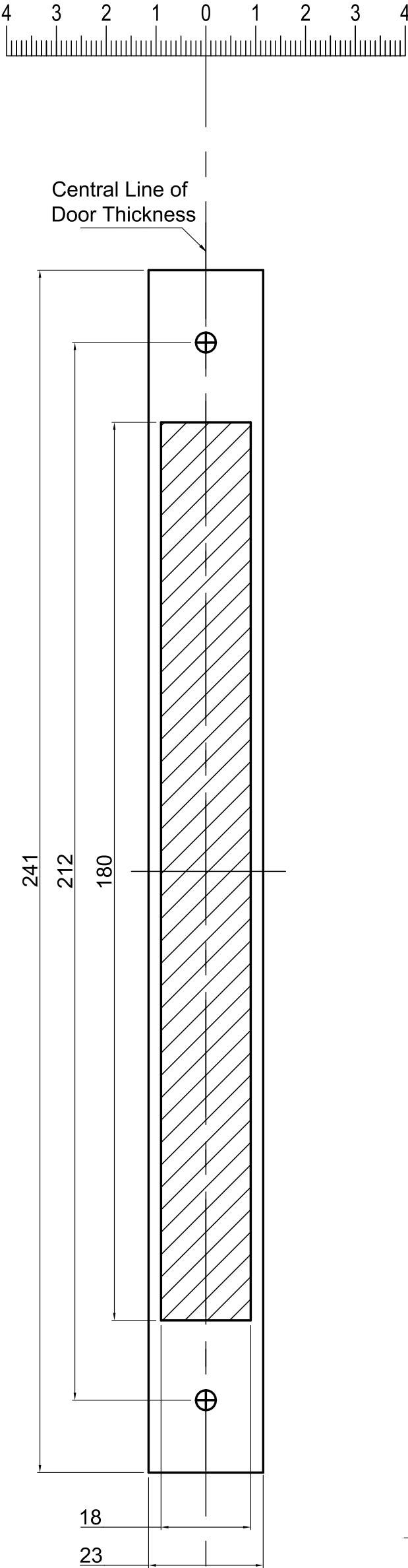
Template For Mortise
