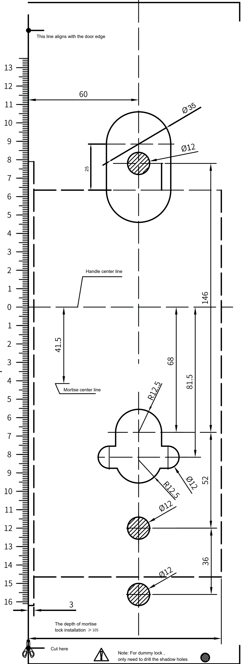
Drill drawing of door leaf
