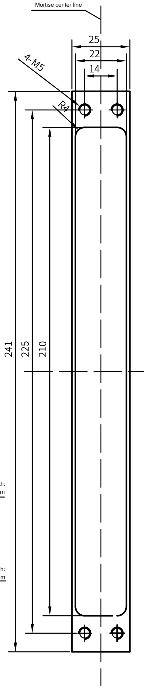
Drill drawing of mortise lock
